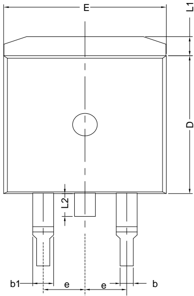
TO-220FJD-3L
