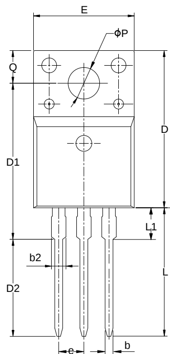
TO-220FJD-3L
