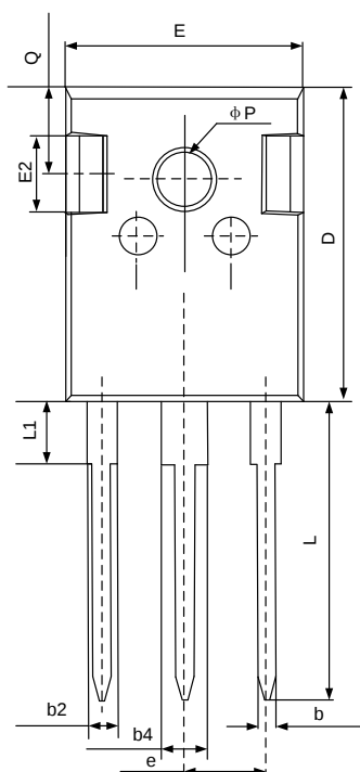
TO-220FJD-3L
